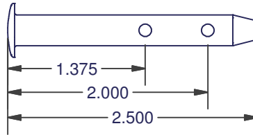
23721 ZINC RESISTANT
