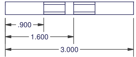
244 STAMPED COMMERCIAL
