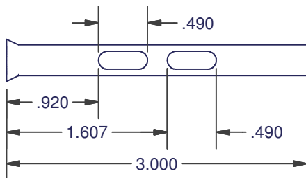
266 STAMPED
