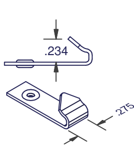
135 GOOSENECK CORD CLIP KNOT-RELIEF REQUIRED
