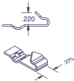
147 TENSION CORD CLIP
