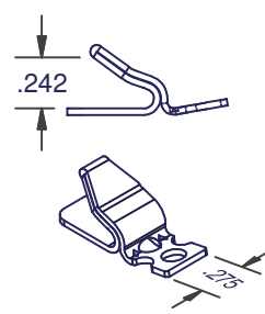
5058 TENSION CORD CLIP USE EXTENDED TRAVEL GUIDES ONLY
