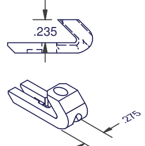
50522 ZINC CORD CLIP
