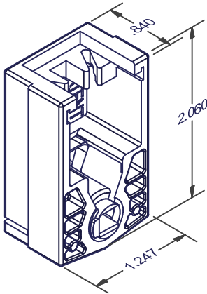
71258 METAL SPRING / SIDE LOCKING
