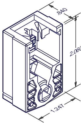
71478 METAL SPRING / SIDE LOCKING
